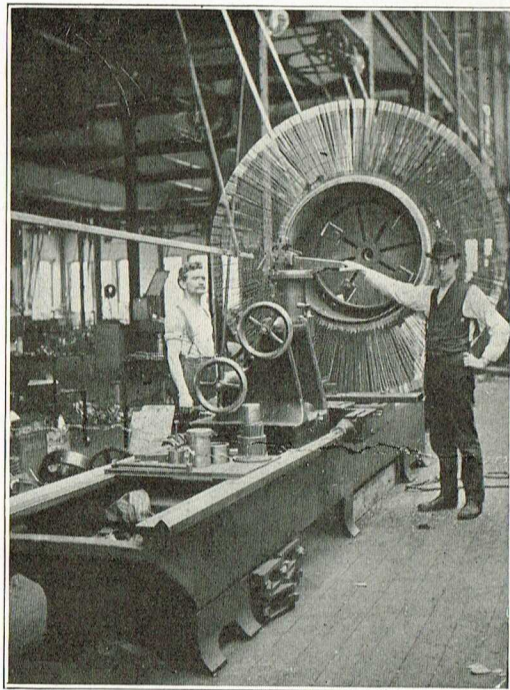
An old-time 504 bar commutator being prepared at the South Shops on July 15, 1904. Foreman J. Seaman is on the right and J. Ambrose, machinist, on the left.
