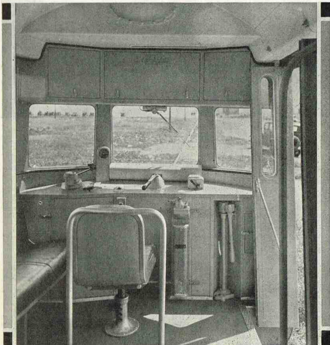
MOTORMAN'S QUARTERS ON MODEL CAR PROVIDE COMFORT, CONVENIENCE AND CLEAR VISION
