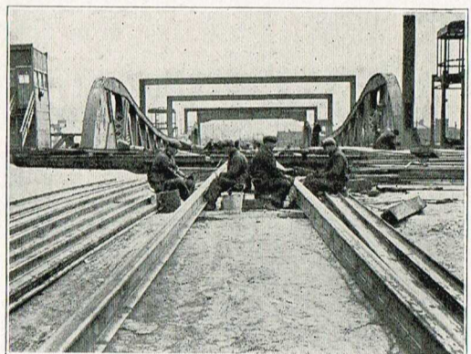
Steel rails being installed on Ashland Avenue structure.
